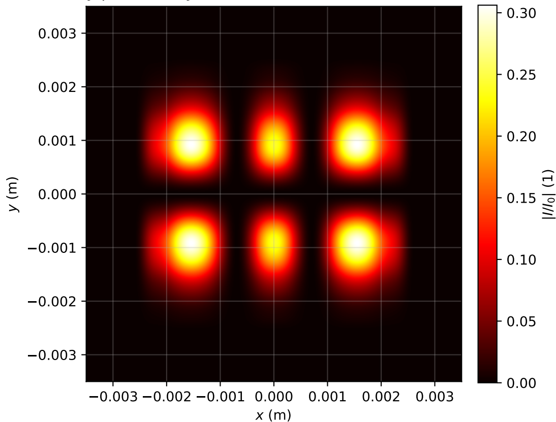
Intensity profile I(x, y, z = 3.344)/I_0 , P_{in}=1.0P_{cr} , artificial time
